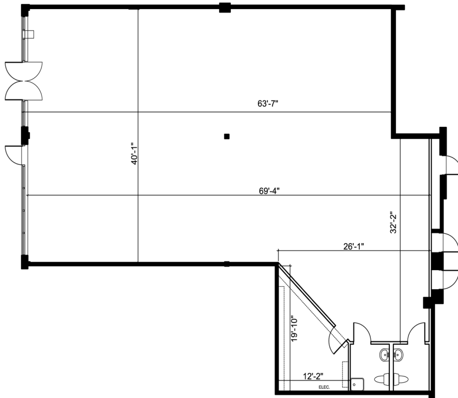
KEY PLAN
